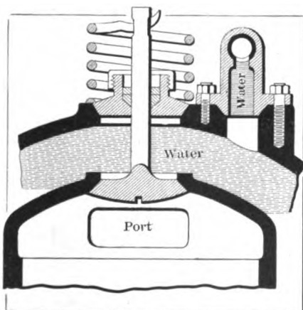
Fig. 32—Differences in expansion compensated for by using springs to hold covers in place.
